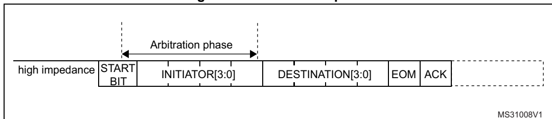
Figure 527. Arbitration phase
