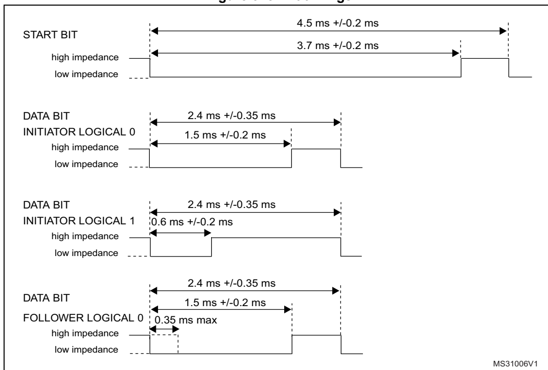
Figure 525. Bit timings
