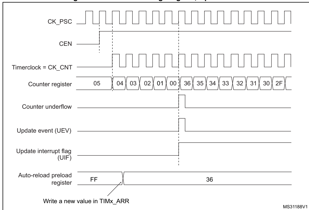
Figure 216. Counter timing diagram, Update event
