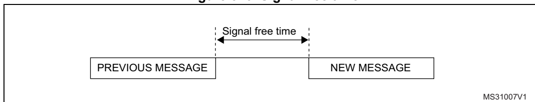
Figure 526. Signal free time
