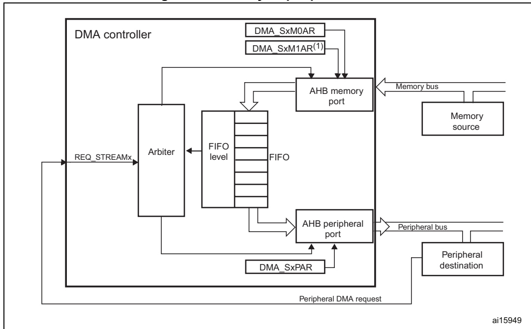
Figure 26. Memory-to-peripheral mode
