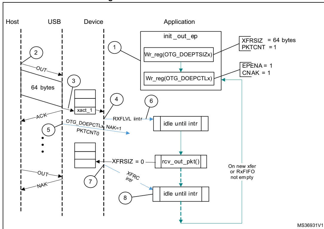
Figure 480. Bulk OUT transaction
